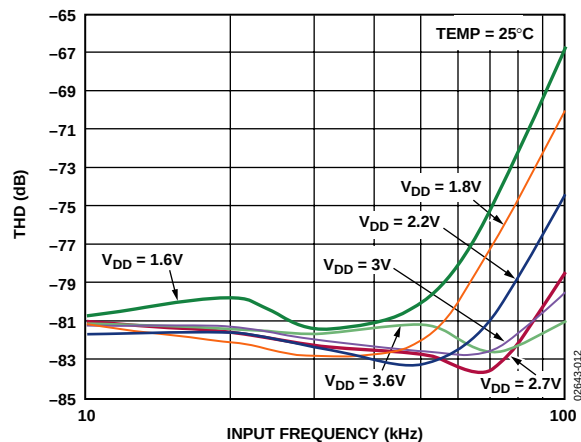
Figure 11. AD7466 THD vs. Analog Input Frequency at 100 kSPS for Various Supply Voltages
