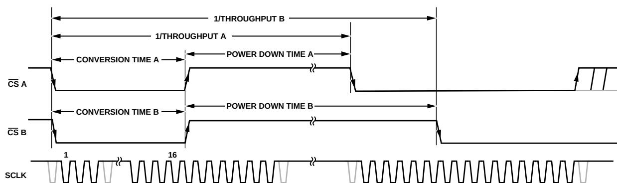
Figure 27. Conversion Time vs. Power-Down Time for a Fixed SCLK Frequency and Different Throughput Rates
