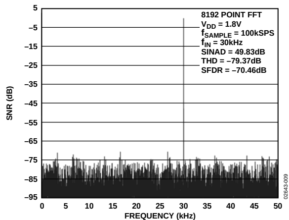
Figure 8. AD7468 Dynamic Performance at 100 kSPS
