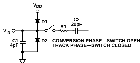
Figure 23. Equivalent Analog Input Circuit
