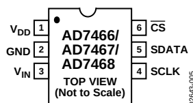
Figure 4. SOT-23 Pin Configuration
