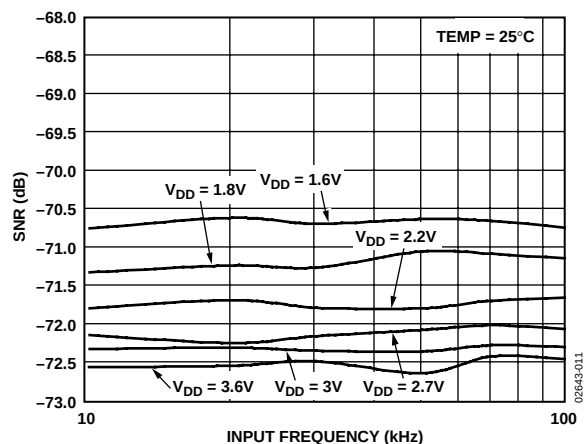
Figure 10. AD7466 SNR vs. Analog Input Frequency at 100 kSPS for Various Supply Voltages
