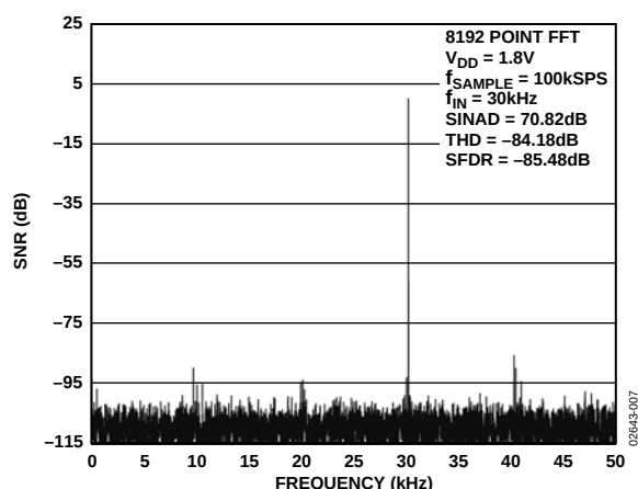
Figure 6. AD7466 Dynamic Performance at 100 kSPS
