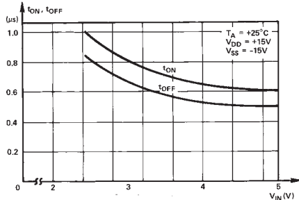
Figure 3. t_{ON} , t_{OFF} vs. Digital Input Voltage
