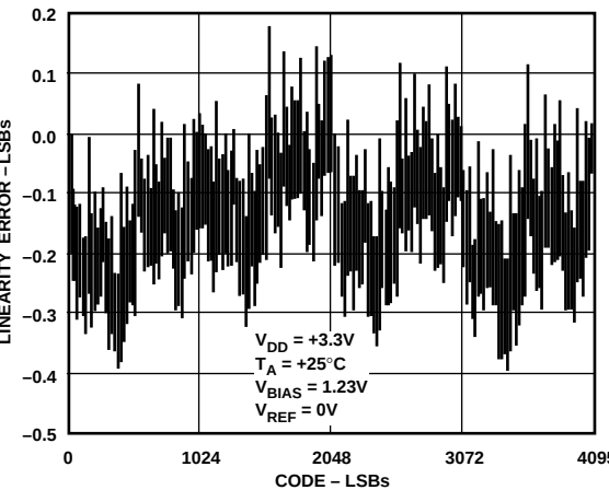
Figure 11. All Codes Linearity Plot (Biased Mode)
