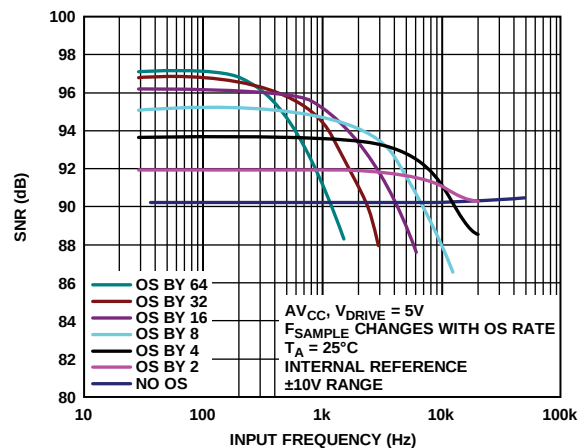
Figure 27. SNR vs. Input Frequency for Different Oversampling Rates, \pm 10V Range
