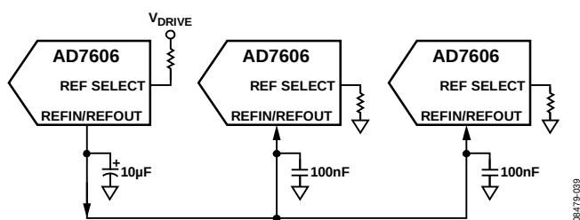
Figure 42. Internal Reference Driving Multiple AD7606-6/AD7606-4 REFIN Pins
