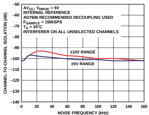
Figure 28. Channel-to-Channel Isolation
