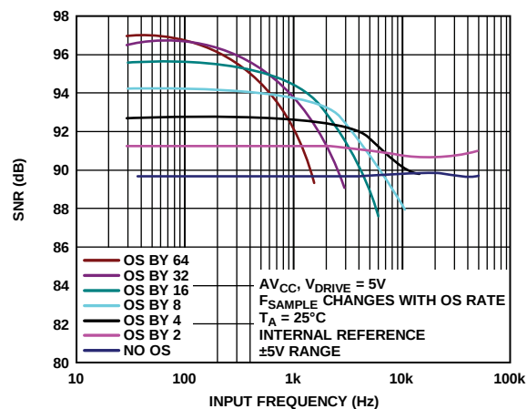
Figure 26. SNR vs. Input Frequency for Different Oversampling Rates, \pm 5V Range
