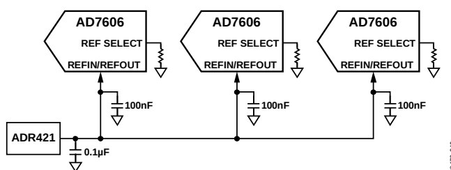
Figure 41. Single External Reference Driving Multiple AD7606-6/AD7606-4 REFIN Pins
