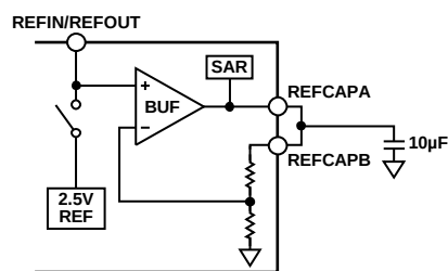
Figure 40. Reference Circuitry
