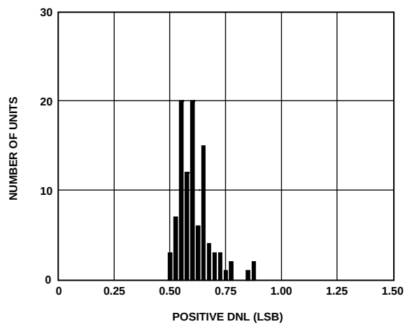
Figure 7. Typical Positive DNL Distribution (99 Units)
