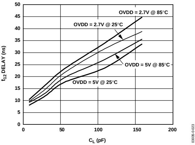
Figure 23. Typical Delay vs. Load Capacitance, C_L
