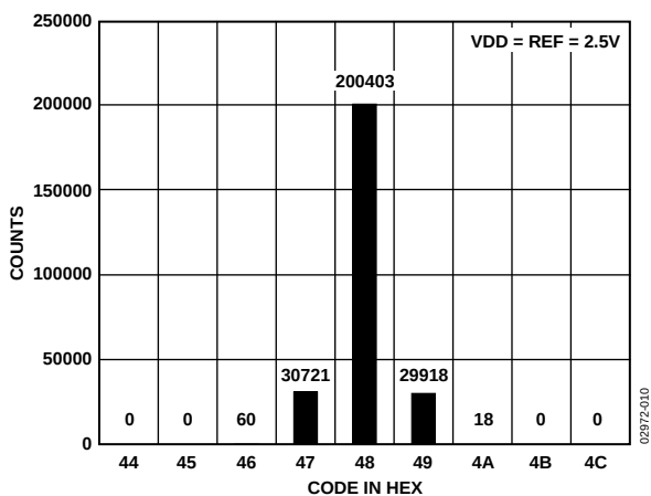
Figure 10. Histogram of a DC Input at the Code Center, VDD = REF = 2.5 V
