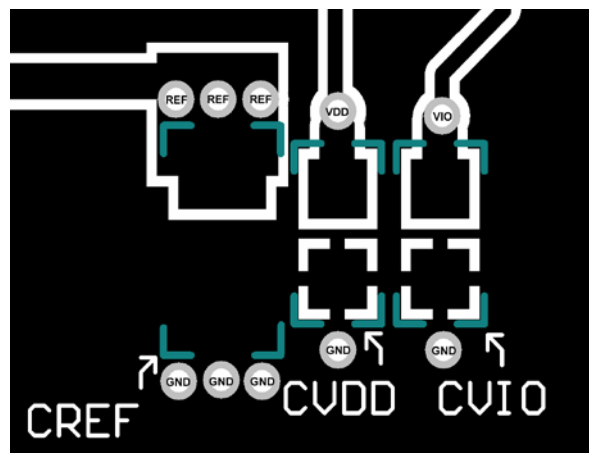
Figure 47. Example of Layout of the AD7687 (Bottom Layer)
