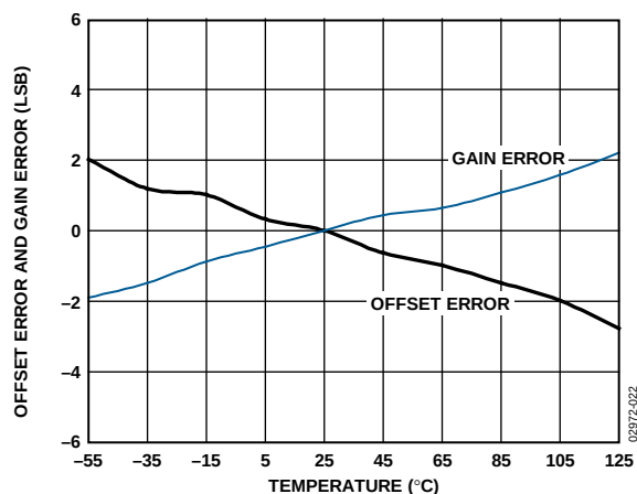
Figure 22. Offset Error and Gain Error vs. Temperature
