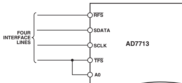
Figure 14. Simplified Interface with \overline{\text{TFS}} Connected to A0
