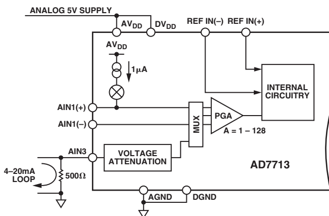
Figure 21. 4–20 mA Measurement Using the AD7713
