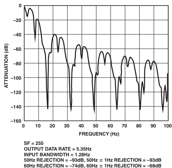
Figure 9. Filter Profile with SF = 255
