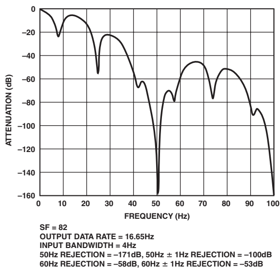
Figure 7. Filter Profile with SF = 82
