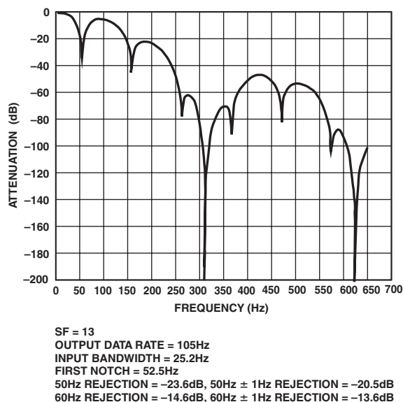
Figure 6. Filter Profile with SF = 13
