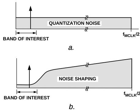
Figure 21. Sigma-Delta ADC
