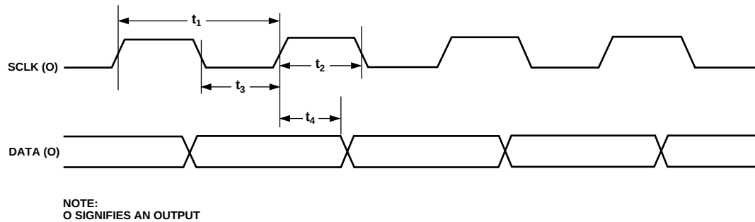
Figure 3. Data Timing
