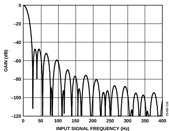
Figure 22. Capacitance Channel Frequency Response, Conversion Time = 109.6 ms
