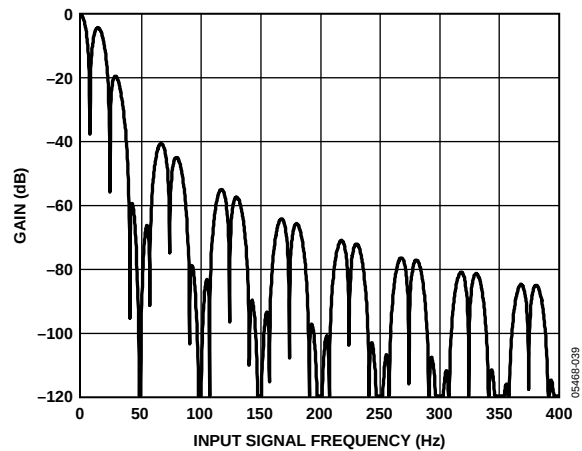
Figure 23. Voltage Channel Frequency Response, Conversion Time = 122.1 ms
