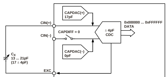
Figure 32. Using CAPDAC in Single-Ended Mode
