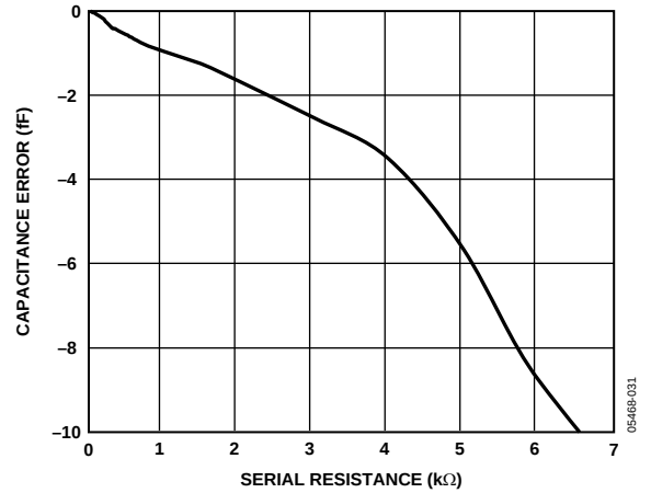
Figure 15. Capacitance Input Error vs. Serial Resistance, C_{IN}(+) to EXC = 21 pF, C_{IN}(-) to EXC = 23 pF, V_{DD} = 5 V, the Same Configuration as in Figure 34.
