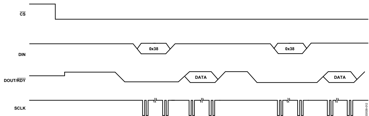
Figure 12. Continuous-Conversion Mode
