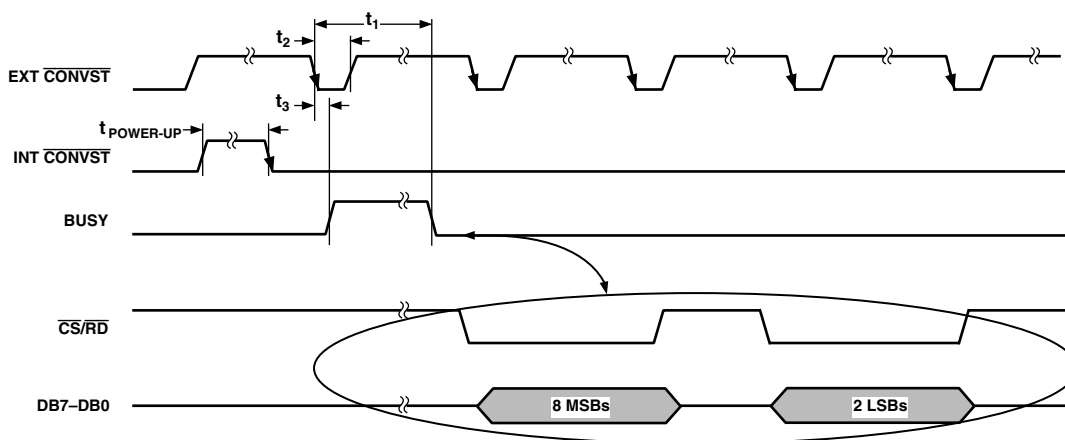
Figure 13. Mode 1 Operation
