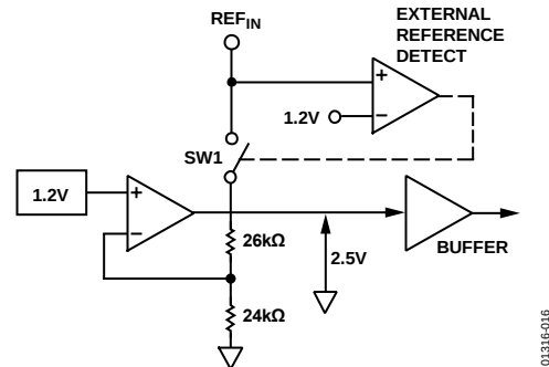
Figure 11. On-Chip Reference
