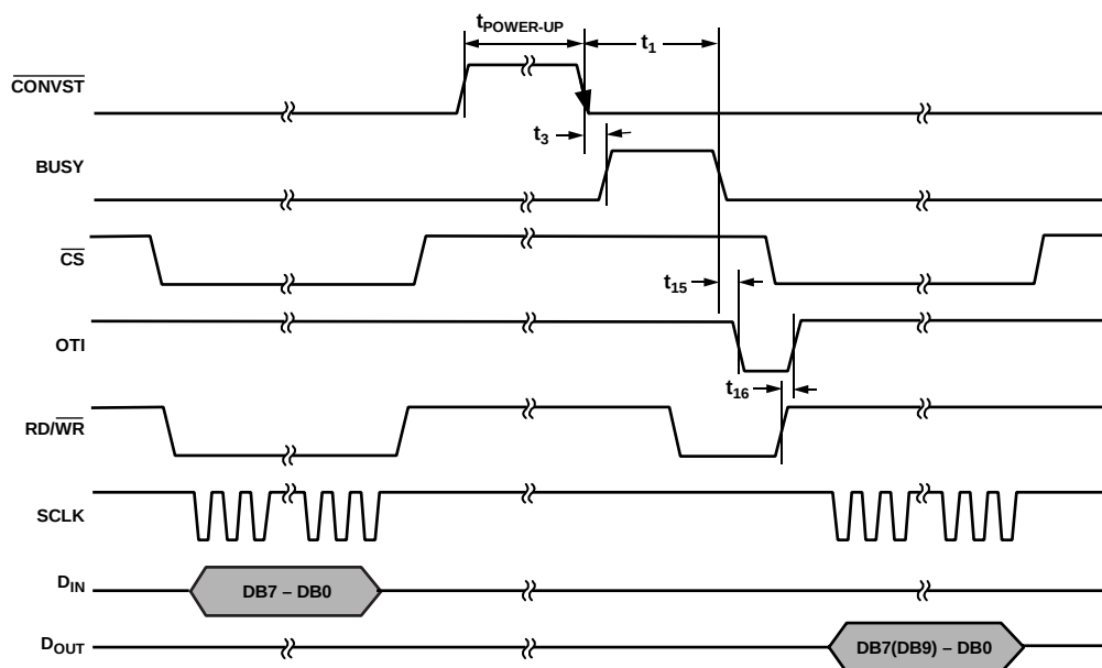
Figure 18. Mode 2 Operation
