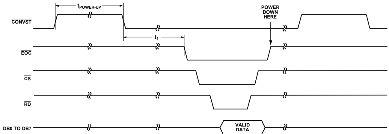
Figure 25. Mode 2 Operation
