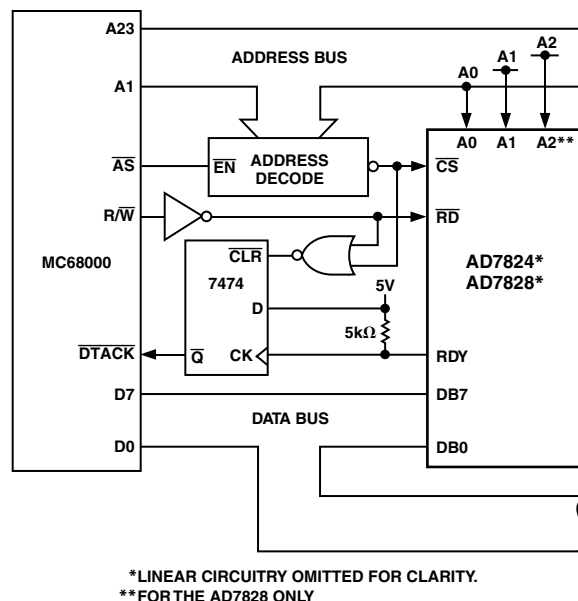
Figure 17. AD7824/AD7828–MC68000 Interface
