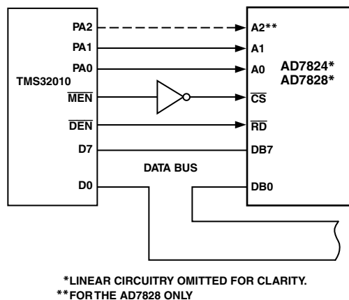
Figure 18. AD7824/AD7828–TMS32010 Interface
