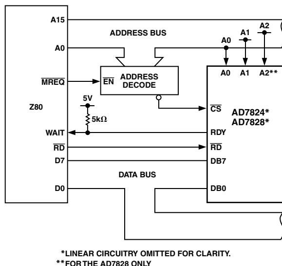
Figure 16. AD7824/AD7828–Z80 Interface
