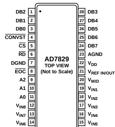
Figure 5. Pin Configuration
