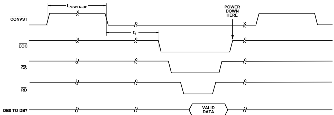
Figure 22. Mode 2 Operation
