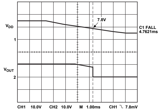
Figure 13. Turn-Off Characteristics
