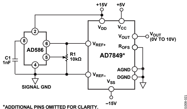
Figure 20. Unipolar Binary Operation
