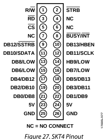
Figure 27. SKT4 Pinout
