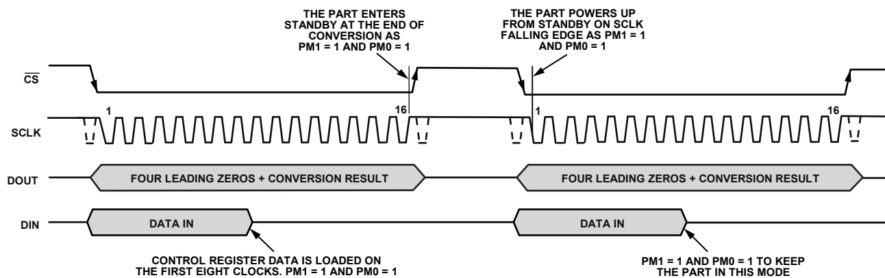
Figure 20. Mode 4 Operation
