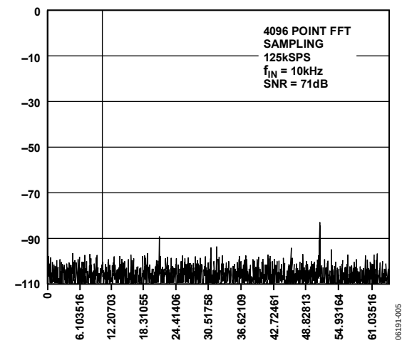
Figure 5. Dynamic Performance
