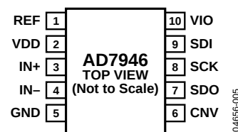
Figure 5. 10-Lead QFN¹ (LFCSP) Pin Configuration
