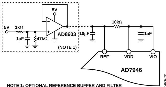
Figure 31. Example of Application Circuit
