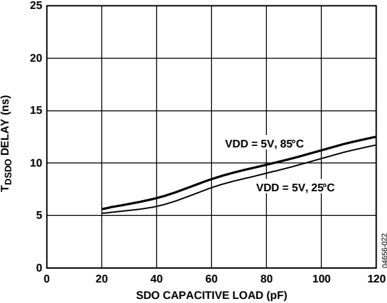
Figure 22. t_{\text{DSDO}} Delay vs. Capacitance Load and Supply
