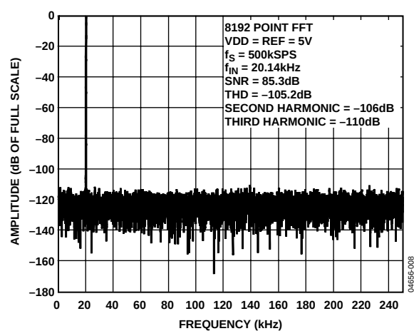
Figure 8. FFT Plot
