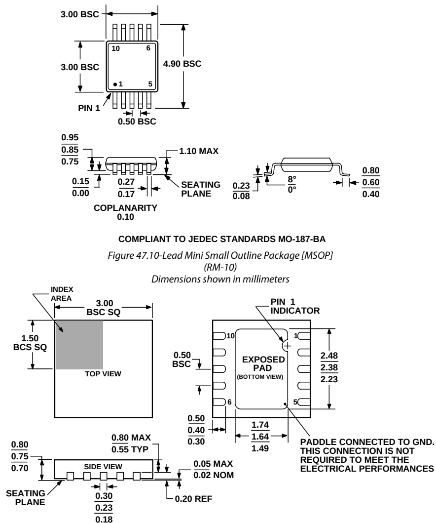
Figure 48. 10-Lead Lead Frame Chip Scale Package [QFN 1 (LFCSP_WD)] 3 mm × 3 mm Body, Very Very Thin, Dual Lead (CP-10-9) Dimensions shown in millimeters
