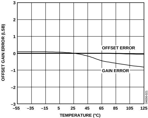
Figure 21. Offset Gain Error vs. Temperature
