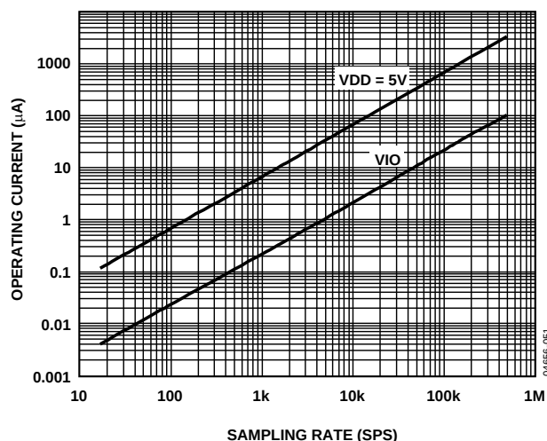
Figure 30. Operating Currents vs. Sampling Rate
