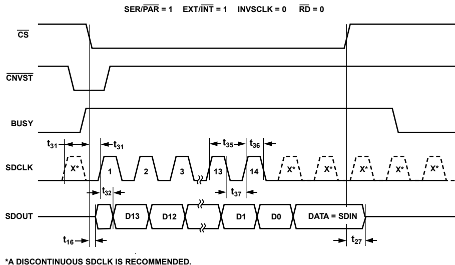
Figure 44. Slave Serial Data Timing for Reading (Read Previous Conversion During Convert)
