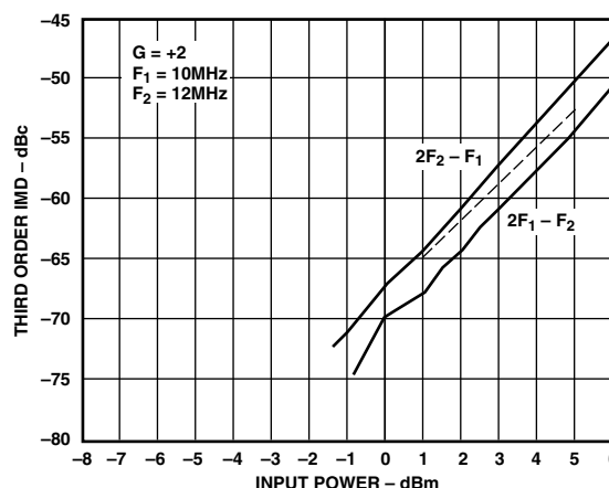
Figure 8. Third Order IMD; F_1 = 10 \text{ MHz} , F_2 = 12 \text{ MHz}
