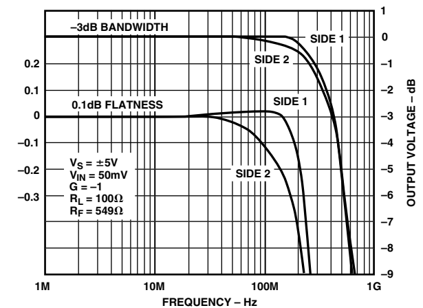
TPC 29. -3 dB Bandwidth vs. Frequency, G = -1
