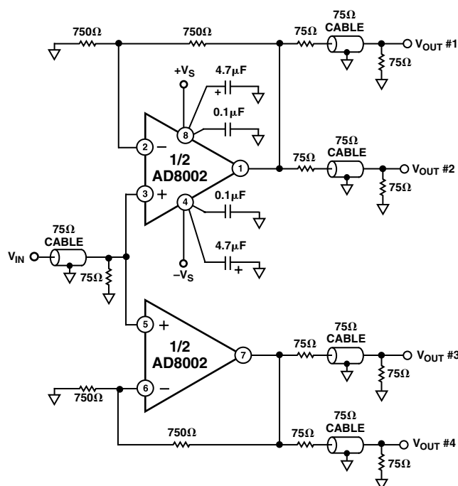
Figure 9. Video Line Driver
