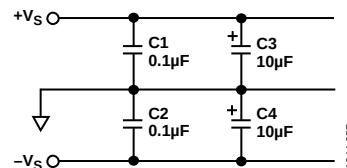
Figure 58. Supply Bypassing
