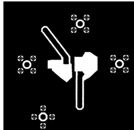
Figure 71. Noninverter MSOP Board Layout (Solder Side) (Looking Through the Board)
