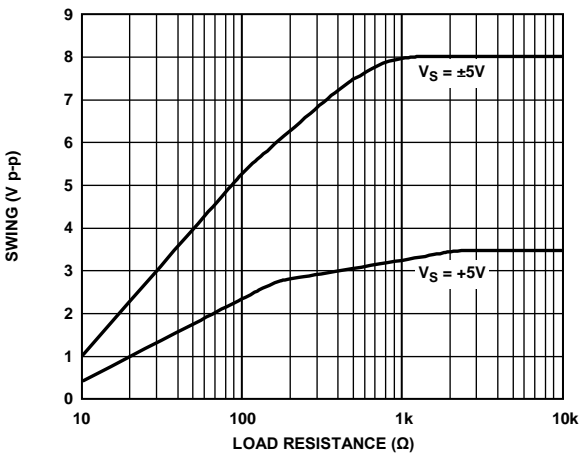
Figure 14. Output Voltage Swing vs. Load
