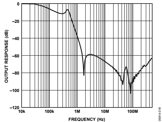
Figure 31. Power Supply Filter Frequency Response in a 50 \Omega System
