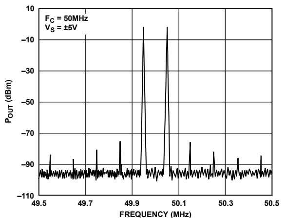
Figure 19. Intermodulation Distortion
