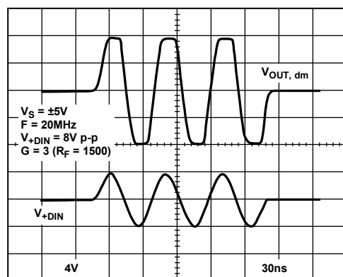
Figure 26. Output Overdrive
