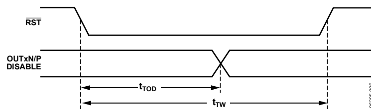
Figure 6. Asynchronous Reset
