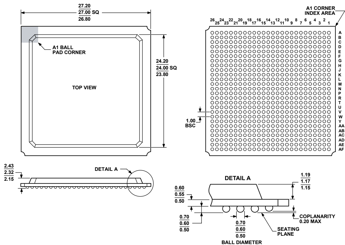
COMPLIANT TO JEDEC STANDARDS MS-034-AAL-1 Figure 54. 676-Ball Plastic Ball Grid Array [PBGA] (B-676) Dimensions shown in millimeters
