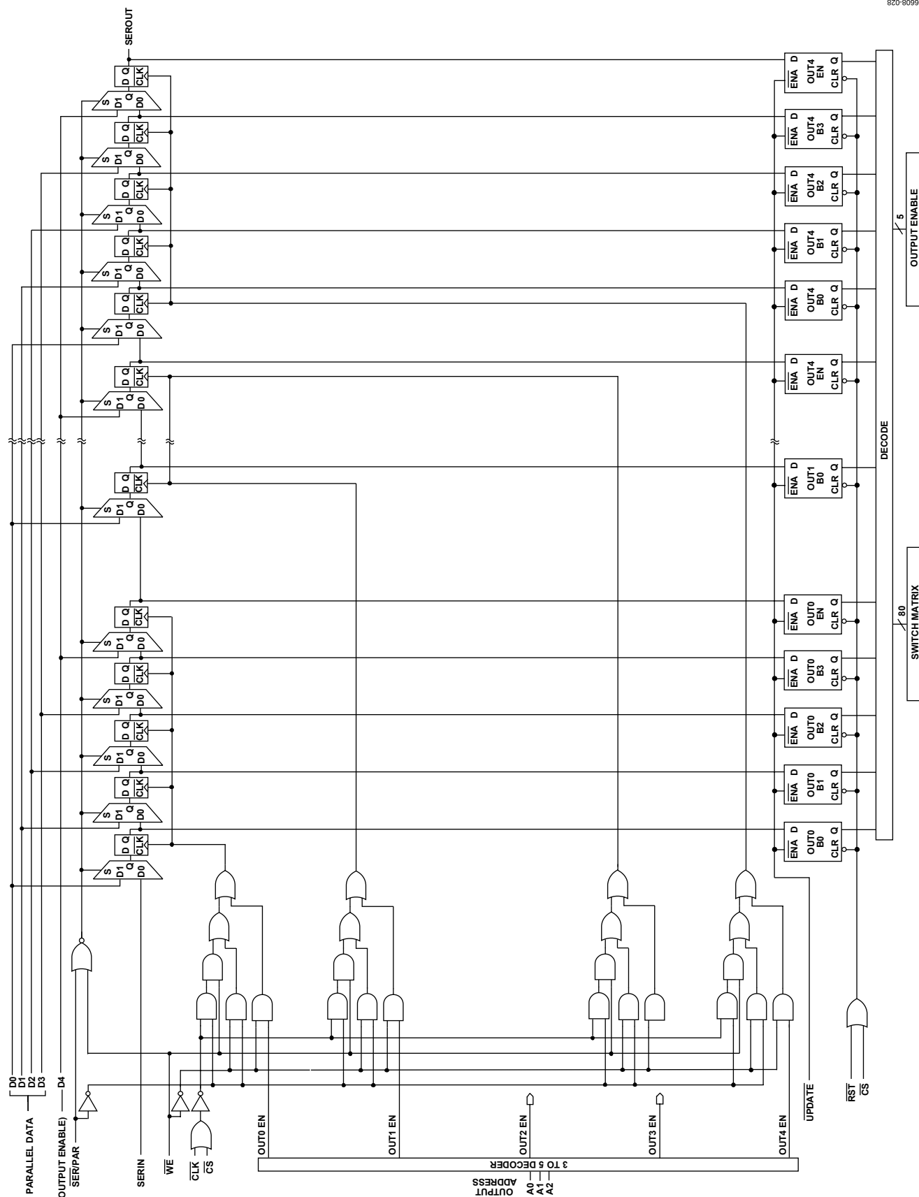
Figure 7. Logic Diagram
