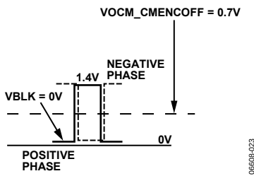
Figure 48. Output at the AD8178 Pins for 0 V to 0.7 V Input Differential Pulse, V_{BLK} = 0\text{ V} , V_{OCM\_CMENCOFF} = 0.7\text{ V}
