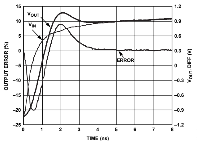
Figure 25. Settling Time
