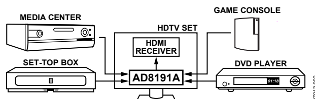
Figure 2. Typical HDTV Application
