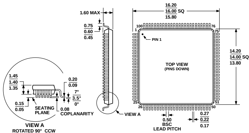
Figure 35. 100-Lead Low Profile Quad Flat Package [LQFP] (ST-100) Dimensions shown in millimeters
