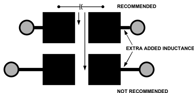
Figure 23. Recommended Pad Outline for Bypass Capacitors
