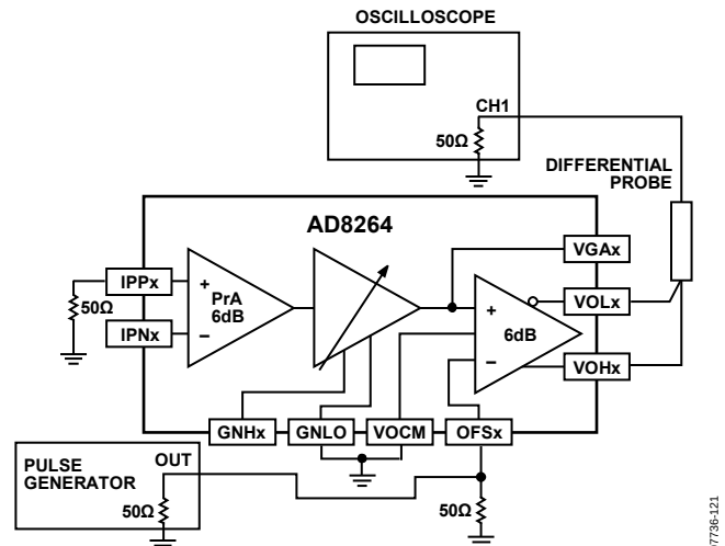
Figure 102. V_{OFSx} Pulse Response (See Figure 60)
