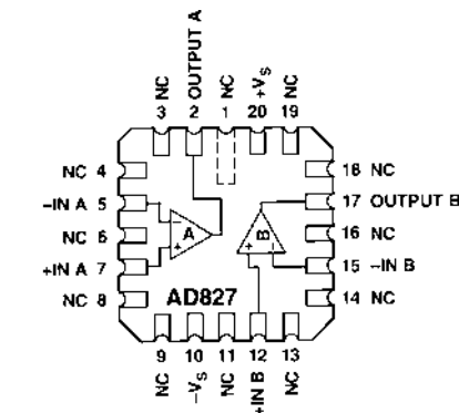
20-Lead LCC (E) Package
