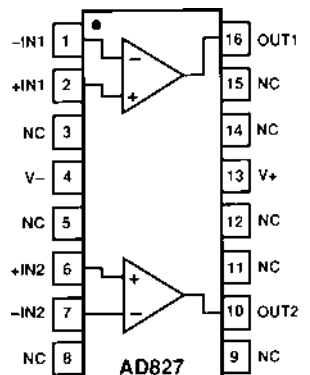
16-Lead Small Outline (R) Package
