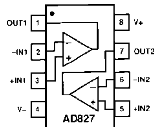
8-Lead Plastic (N) and Cerdip (Q) Packages
