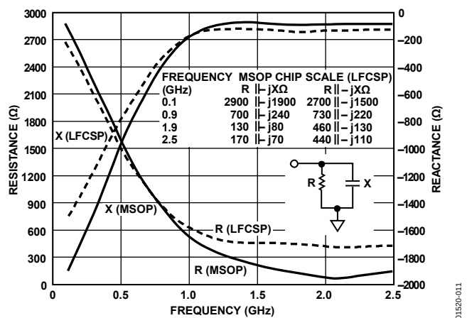
Figure 11. Input Impedance
