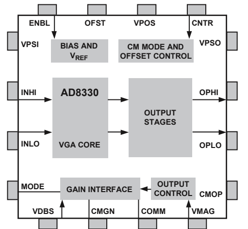
Figure 46. Block Schematic
