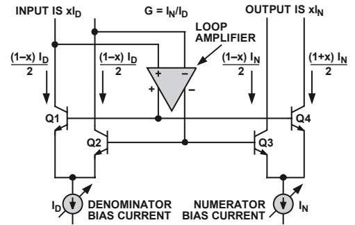
Figure 45. Basic Core
