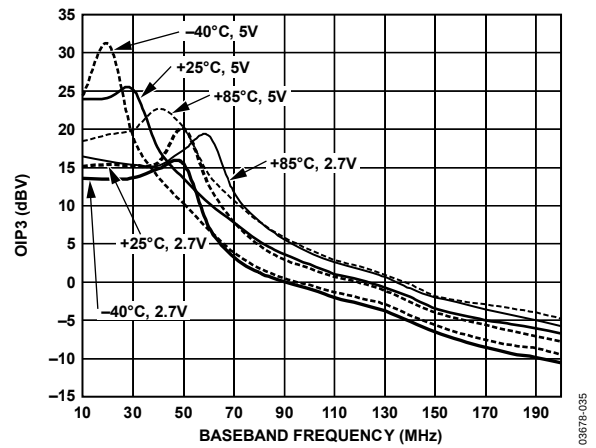
Figure 35. OIP3 vs. F_{BB} , V_{VCMO} = V_{REF} = 1\text{ V} , V_{POS} = 2.7\text{ V}, 5\text{ V} , Temperature = -40^{\circ}\text{C} , +25^{\circ}\text{C} , +85^{\circ}\text{C}
