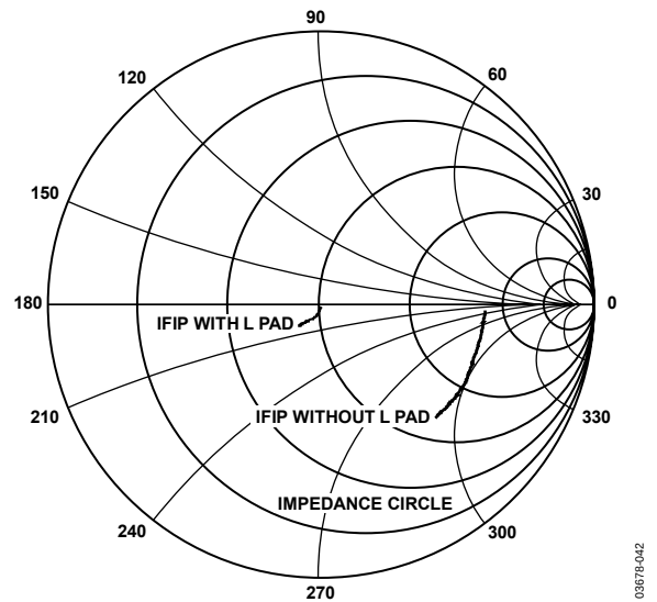
Figure 42. S_{11} of IF Input vs. F_{IF} , F_{IF} = 50\text{ MHz} to 1\text{ GHz} , V_{GIN} = 0.7\text{ V} , V_{POS} = 5\text{ V} (with L Pad, with No Pad, Normalized to 50\text{ }\Omega )
