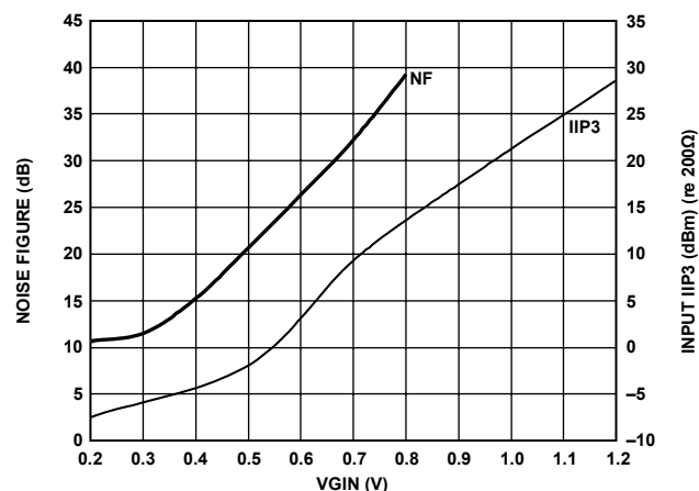
Figure 27. Noise Figure and IIP3 vs. V_{GIN} , Temperature = 25^\circ\text{C} , F_{IF} = 380\text{ MHz} , F_{BB} = 1\text{ MHz} , V_{POS} = 2.7\text{ V}
