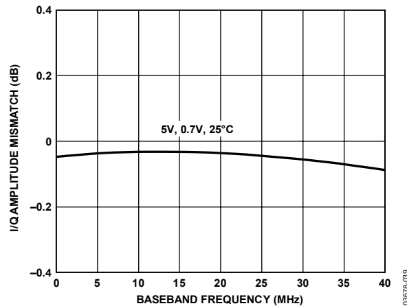
Figure 39. I/Q Amplitude Imbalance vs. F_{BB} , Temperature = 25^{\circ}\text{C} , V_{POS} = 5\text{ V}
