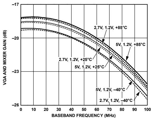
Figure 19. Gain vs. F_{BB} , V_{GIN} = 1.2\text{ V} , F_{IF} = 380\text{ MHz} , V_{POS} = 2.7\text{ V} , 5\text{ V} , Temperature = -40^\circ\text{C} , +25^\circ\text{C} , +85^\circ\text{C}
