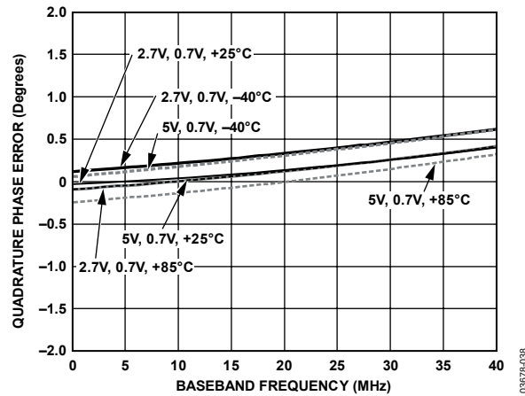
Figure 38. Quadrature Phase Error vs. F_{BB} , V_{GIN} = 0.7\text{ V} , V_{POS} = 2.7\text{ V} , 5\text{ V} , Temperature = -40^{\circ}\text{C} , +25^{\circ}\text{C} , +85^{\circ}\text{C} , F_{IF} = 380\text{ MHz}
