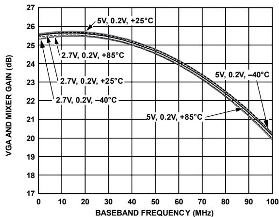
Figure 18. Gain vs. F_{BB} , V_{GIN} = 0.2\text{ V} , F_{IF} = 380\text{ MHz} , V_{POS} = 2.7\text{ V} , 5\text{ V} , Temperature = -40^\circ\text{C} , +25^\circ\text{C} , +85^\circ\text{C}
