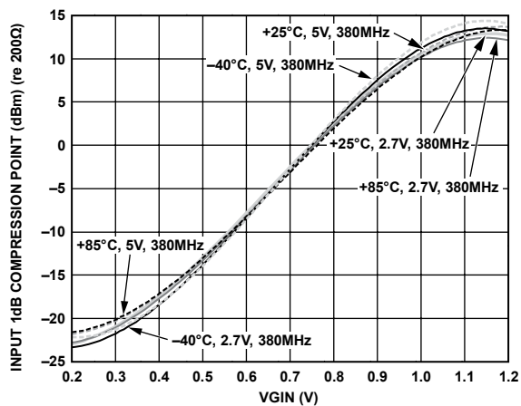
Figure 20. Input 1 dB Compression Point (IP1dB) vs. V_{GIN} , F_{IF} = 380\text{ MHz} , F_{BB} = 1\text{ MHz} , V_{POS} = 2.7\text{ V} , 5\text{ V} , Temperature = -40^\circ\text{C} , +25^\circ\text{C} , +85^\circ\text{C}
