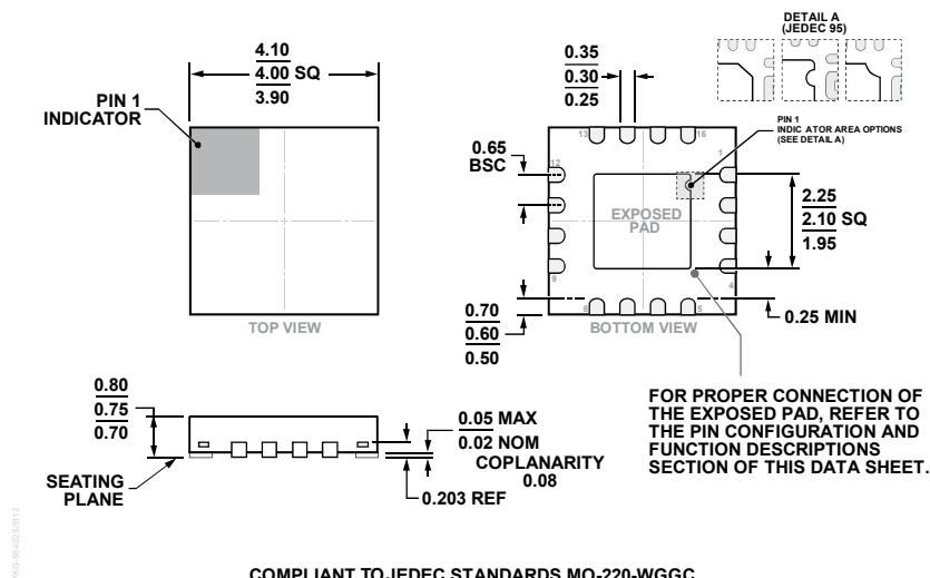
Figure 18. 16-Lead Lead Frame Chip Scale Package (LFCSP) 4 mm × 4 mm Body and 0.75 mm Package Height (CP-16-23)
