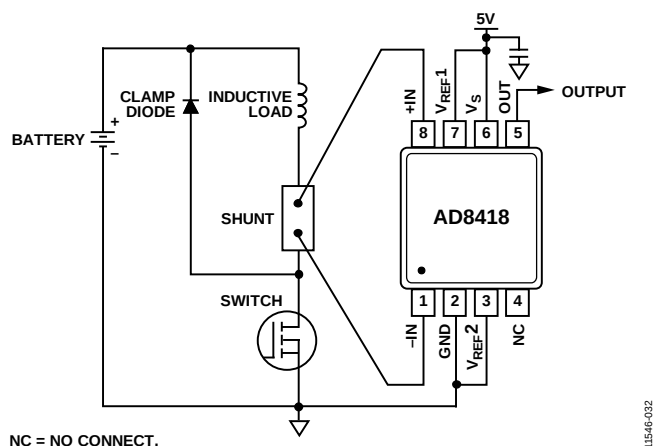
Figure 34. Low-Side Switch
