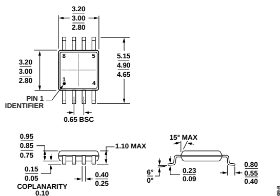
Figure 38. 8-Lead Mini Small Outline Package [MSOP] (RM-8)
