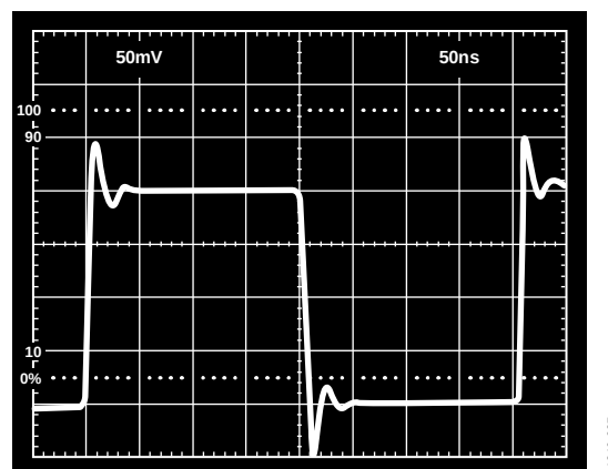
Figure 27. Buffer Small Signal Pulse Response
