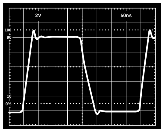
Figure 26. Buffer Large Signal Pulse Response
