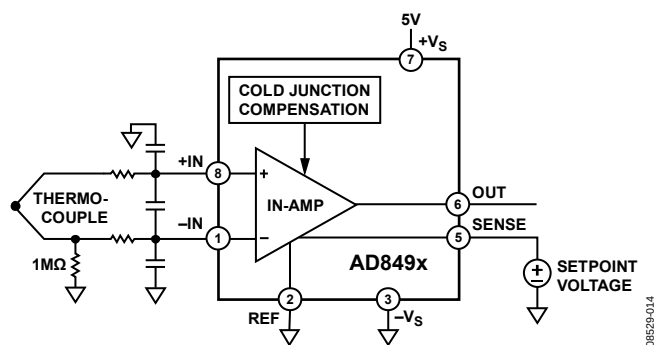
Figure 35. Setpoint Controller
