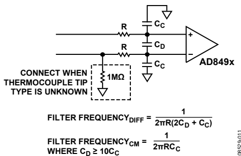
Figure 29. Filter for Any Thermocouple Style
