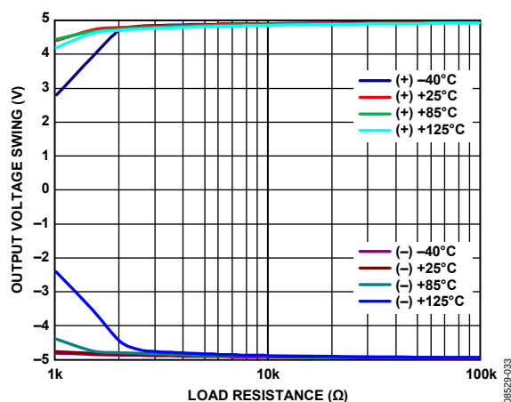
Figure 22. Output Voltage Swing vs. Load Resistance, V_S = \pm 5V
