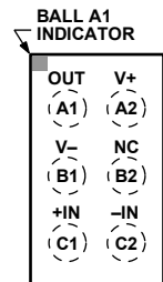
Figure 2. 6-Ball WLCSP (CB-6-7)
