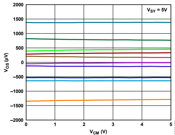
Figure 12. Input Offset Voltage vs. Input Common-Mode Voltage
