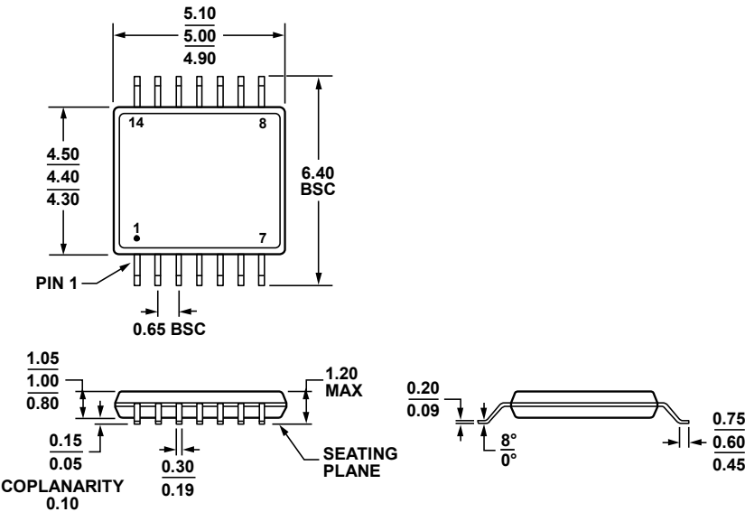
Figure 55. 14-Lead Thin Shrink Small Outline Package [TSSOP] (RU-14) Dimensions shown in millimeters
