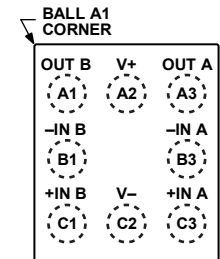
Figure 2. 6-Ball WLCSP (CB-6-7)
