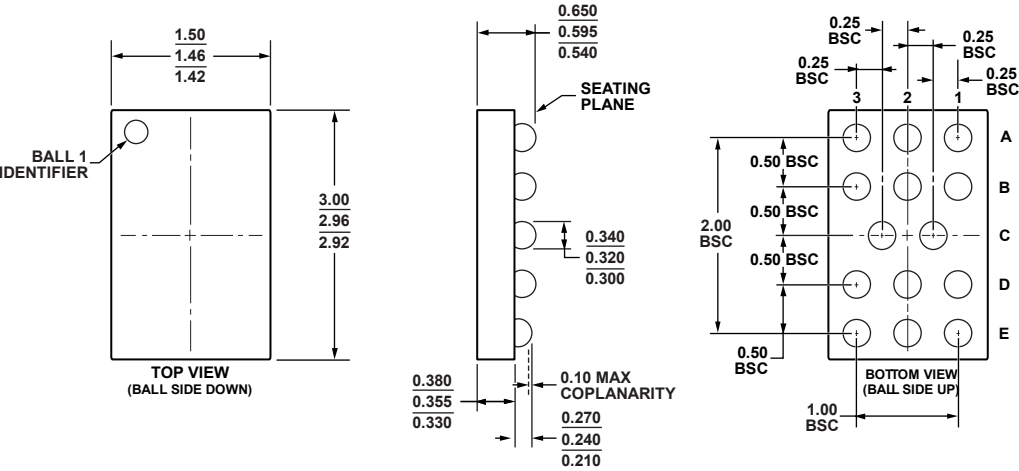
Figure 56. 14-Ball Wafer Level Chip Scale Package [WLCSP] (CB-14-1) Dimensions shown in millimeters
