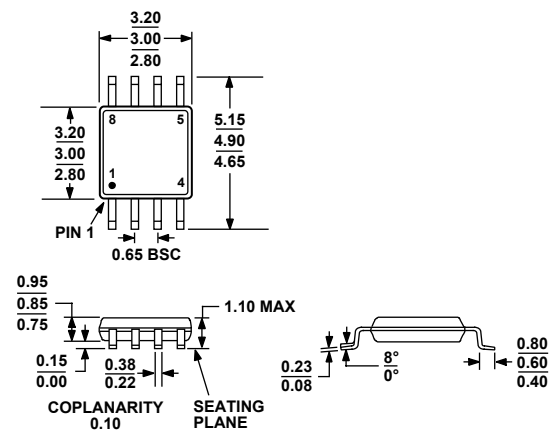
COMPLIANT TO JEDEC STANDARDS MO-187-AA Figure 27. 8-Lead Mini Small Outline Package [MSOP] (RM-8)
