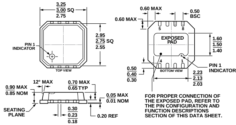
Figure 43. 8-Lead Lead Frame Chip Scale Package [LFCSP_VD] 3 mm × 3 mm Body, Very Thin, Dual Lead (CP-8-9)
