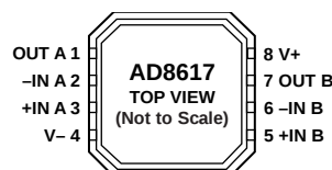
Figure 2. 8-Lead MSOP and 8-Lead SOIC_N
