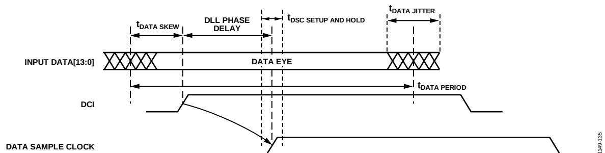
Figure 130. LVDS Data Port Timing Requirements
