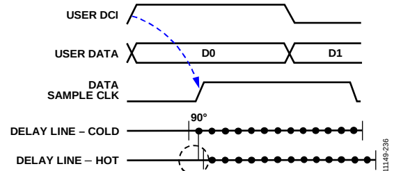
Figure 132. Example of DLL Length Variation Across Temperature
