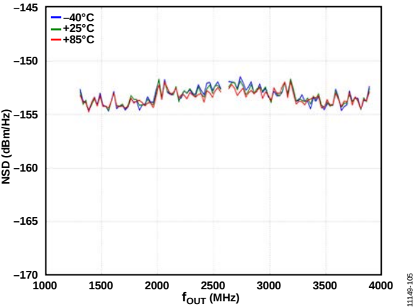
Figure 94. Single-Tone NSD vs. f_{OUT} over Temperature
