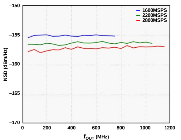
Figure 15. W-CDMA NSD vs. f_{OUT}
