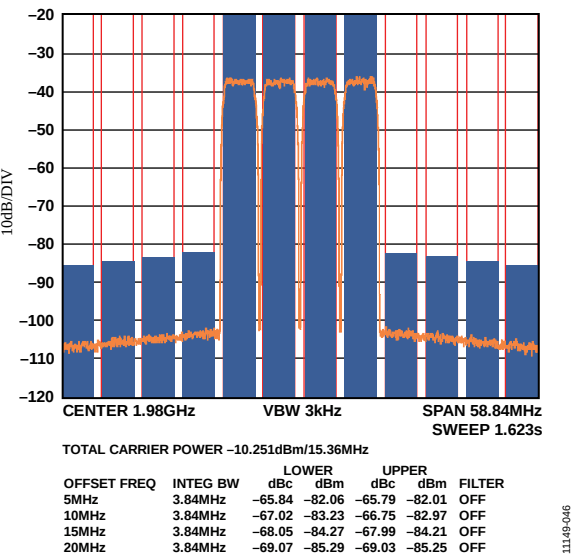
Figure 37. Four-Carrier W-CDMA at 1980 MHz
