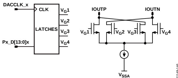
Figure 143. Quad-Switch Architecture
