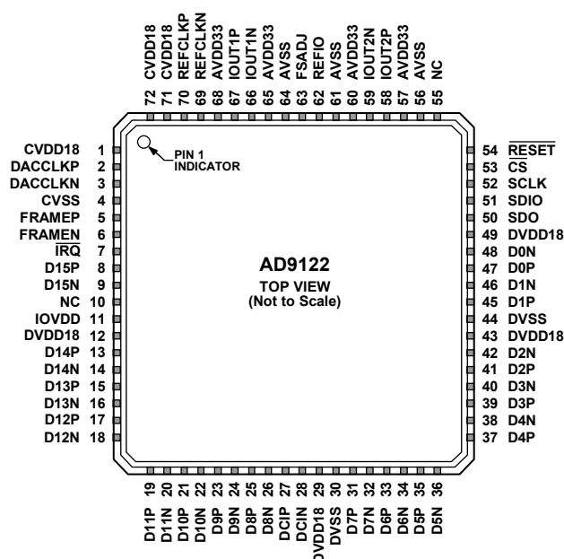
Figure 3. Pin Configuration
