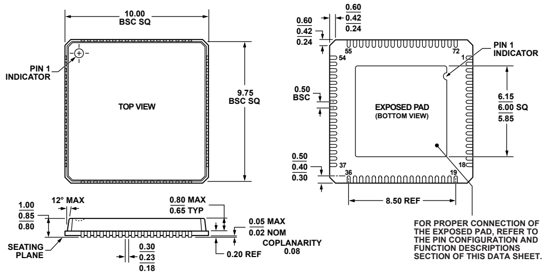
Figure 89. 72-Lead Lead Frame Chip Scale Package [LFCSP_VQ] 10 mm x 10 mm Body, Very Thin Quad (CP-72-7) Dimensions shown in millimeters
