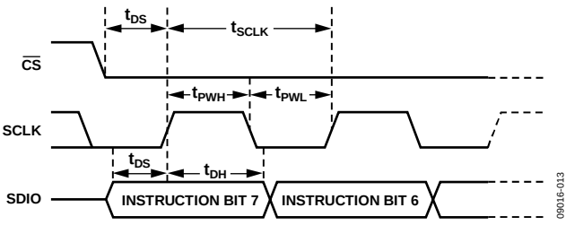
Figure 40. Timing Diagram for Serial Port Register Write ( t_{DS} to t_{DSCS} )
