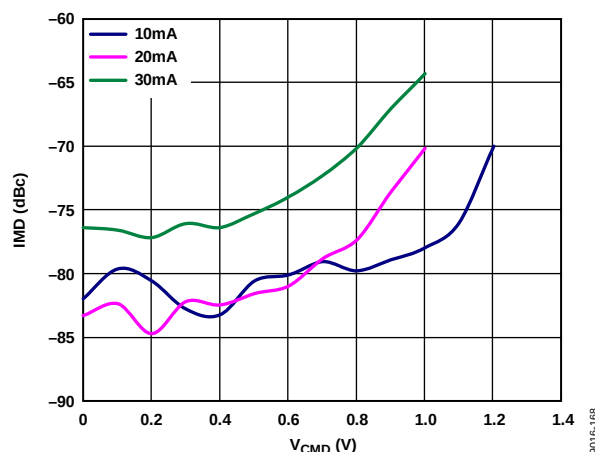
Figure 70. IMD vs. Common-Mode Output Voltage ( f_{OUT} = 61 MHz, R_{LOAD} = 50 \Omega differential, I_{FS} = 10 mA, 20 mA, and 30 mA)
