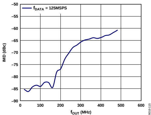
Figure 18. IMD vs. f_{OUT} over f_{DATA} , 8 \times Interpolation, Digital Scale = 0 dBFS, f_{SC} = 20 mA
