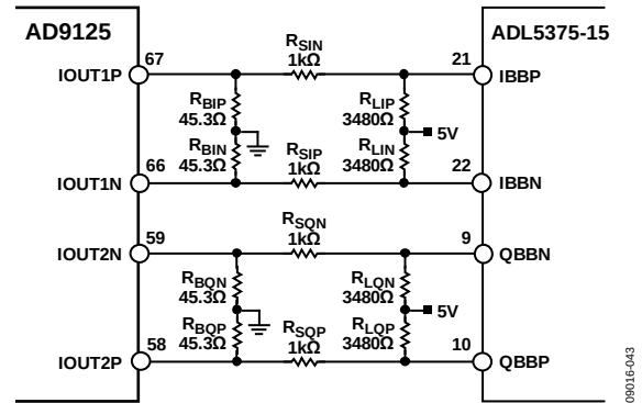
Figure 74. Passive Level-Shifting Network for Biasing ADL5375-15
