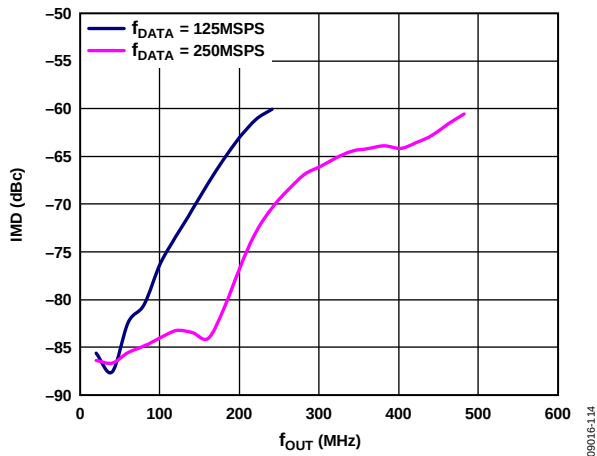
Figure 17. IMD vs. f_{OUT} over f_{DATA} , 4 \times Interpolation, Digital Scale = 0 dBFS, f_{SC} = 20 mA
