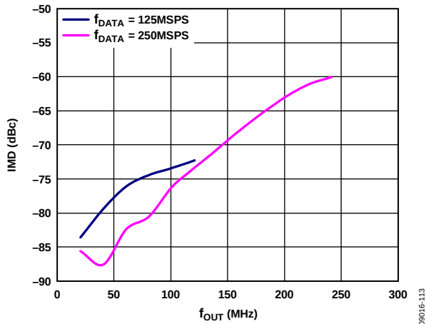
Figure 16. IMD vs. f_{OUT} over f_{DATA} , 2 \times Interpolation, Digital Scale = 0 dBFS, f_{SC} = 20 mA
