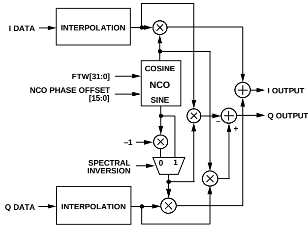
Figure 57. Digital Quadrature Modulator Block Diagram
