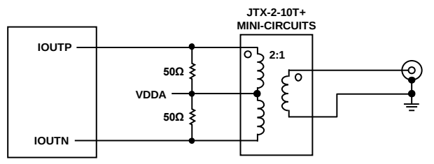
Figure 152. Recommended Transformer for Wideband Applications with Upper Bandwidths of up to 2.2 GHz
