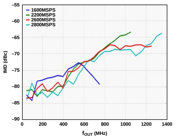
Figure 14. IMD vs. f_{OUT} over f_{DAC}
