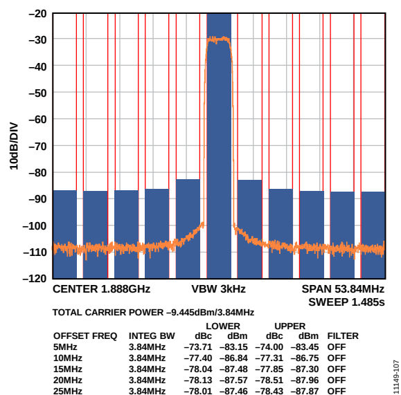
Figure 95. Single-Carrier W-CDMA at 1887.5 MHz
