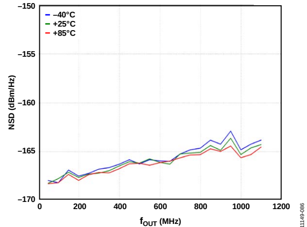
Figure 77. W-CDMA NSD vs. f_{OUT} over Temperature
