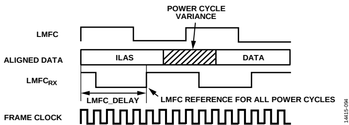
Figure 102. LMFC_DELAY_x to Compensate for Link Delay &gt; LMFC
