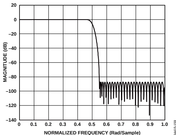
Figure 111. First 2x Half-Band 90% Filter Response
