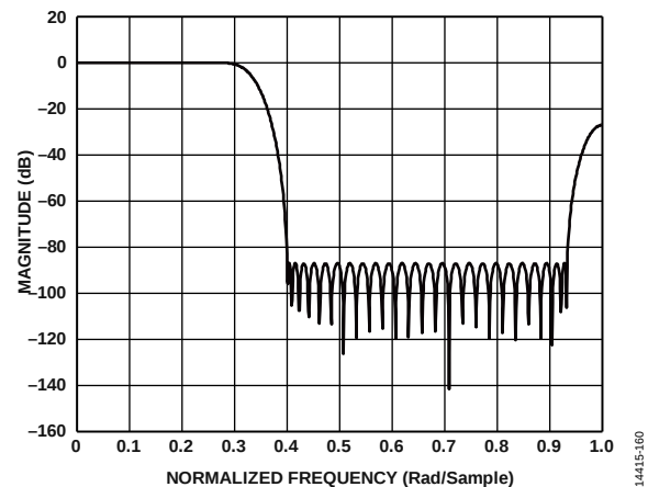
Figure 112. 3x Third-Band 80% Filter Response
