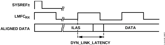
Figure 104. DYN_LINK_LATENCY_x Illustration
